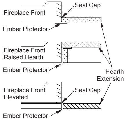
Figure 3 - Hearth Extension
